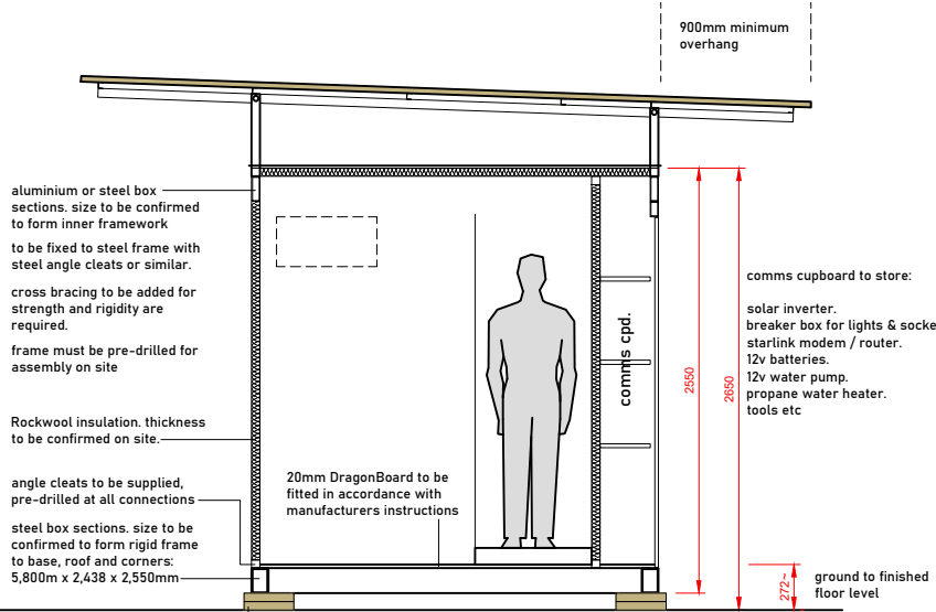
Section
