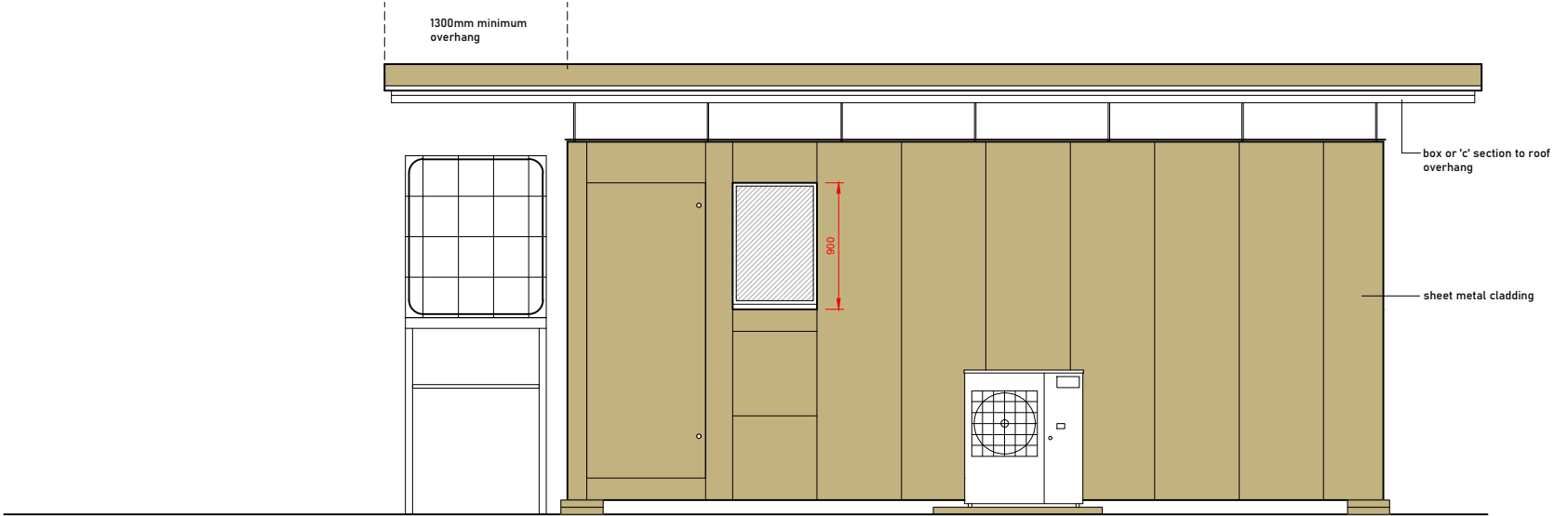
Rear Elevation
